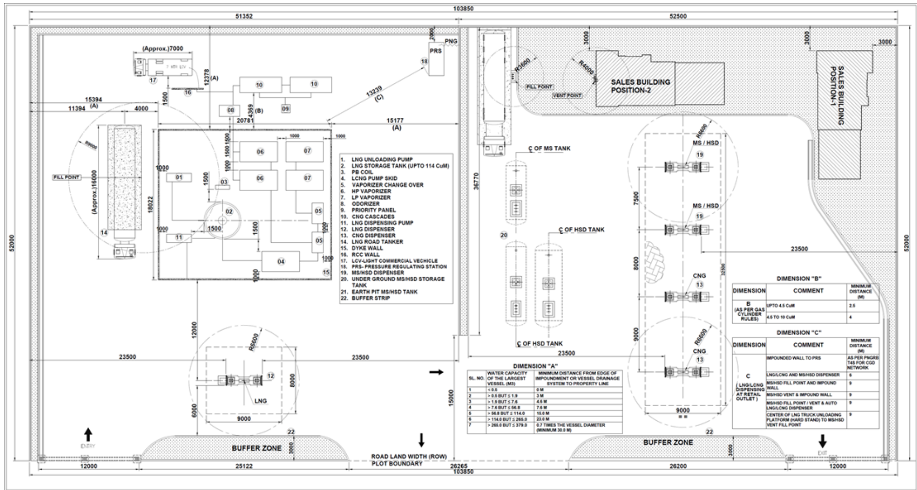
Layout – I. Typical layout of Auto LNG/ LCNG station with provision of mobile cascade filling and PNG
